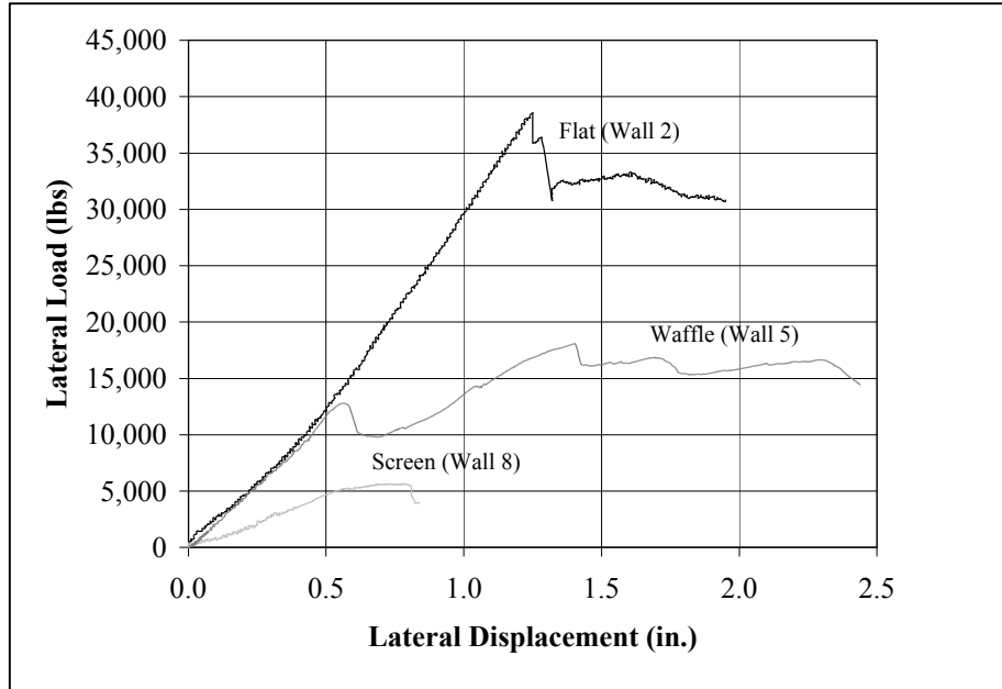
Figure 18 Force-Displacement Response for the 12ft x 8ft with Window Opening ICF Shear Wall Specimens (Wall 2, Wall 5, and Wall 8)
