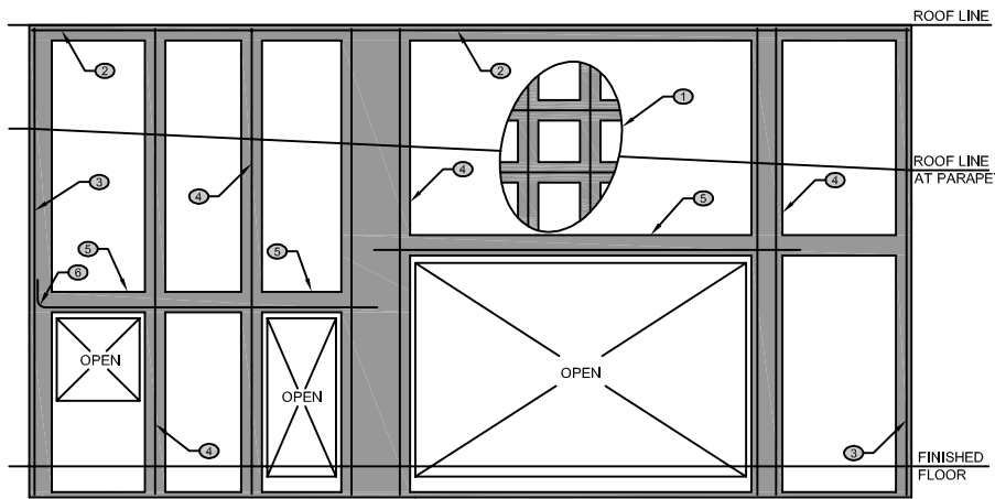
08 TYPICAL ICF SCREEN-GRID PANEL ELEVATION
